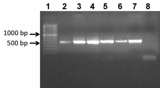
Fig. 1. PCR products of 16S mtDNA gene of grouper species. Lane 1: DNA marker 100 bp. Lane 2–7, PCR products of grouper species. Lane 8: negative control.
